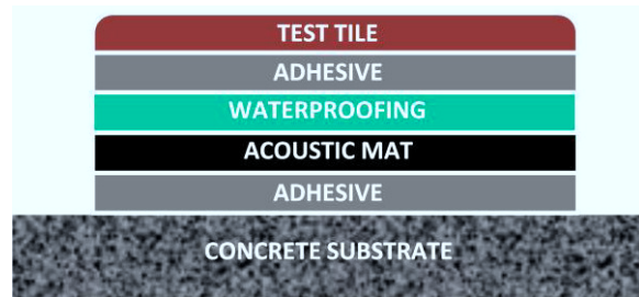
Schematic representation of a wet area test sample.
