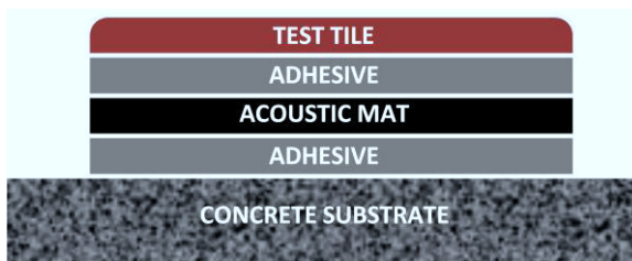
Schematic representation of a dry area test sample.
