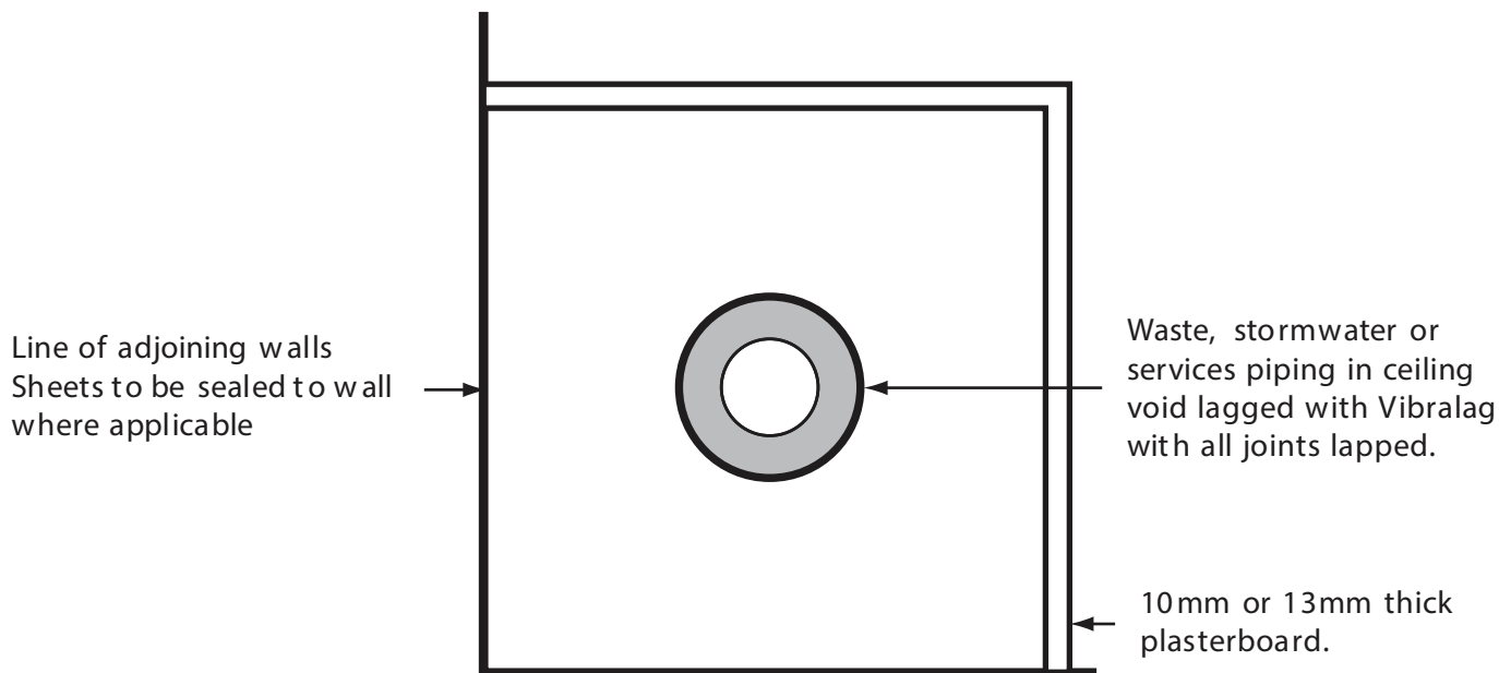
PIPE RISER IN NON-HABITABLE SPACES
