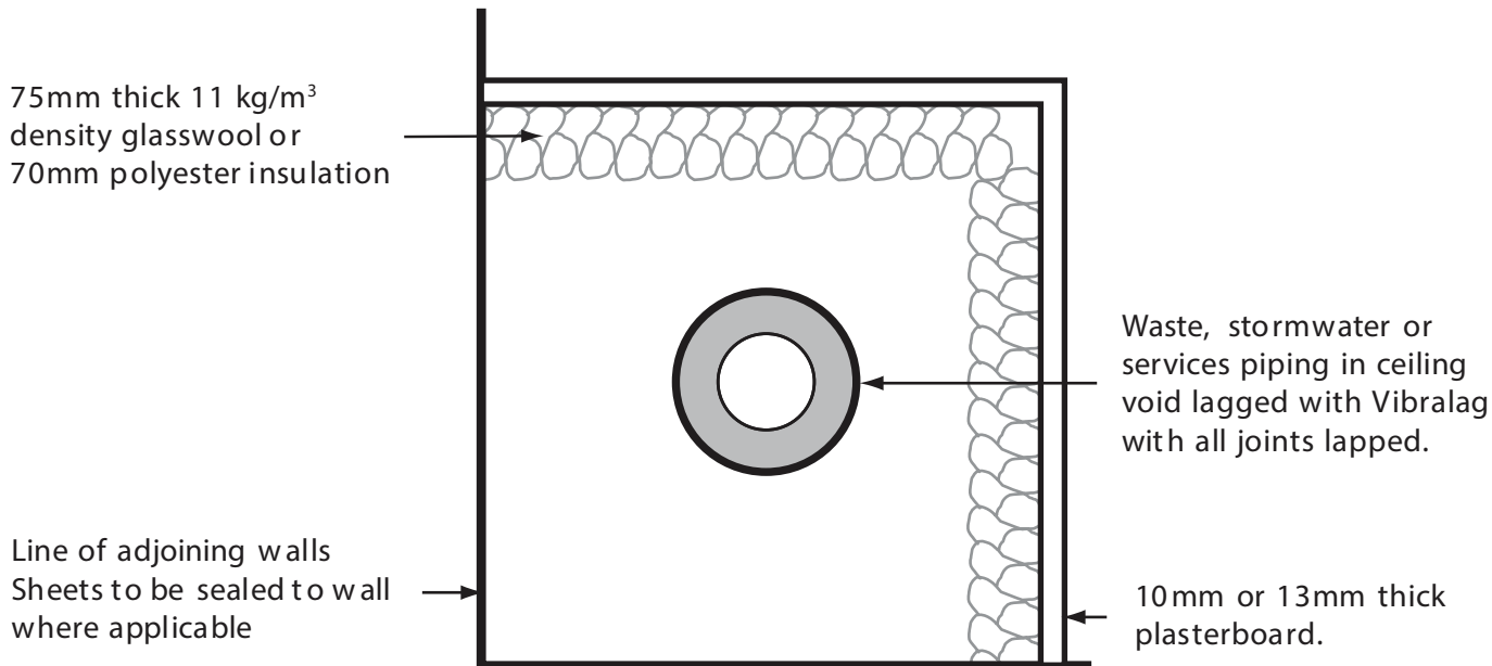
PIPE RISER HABITABLE SPACES
